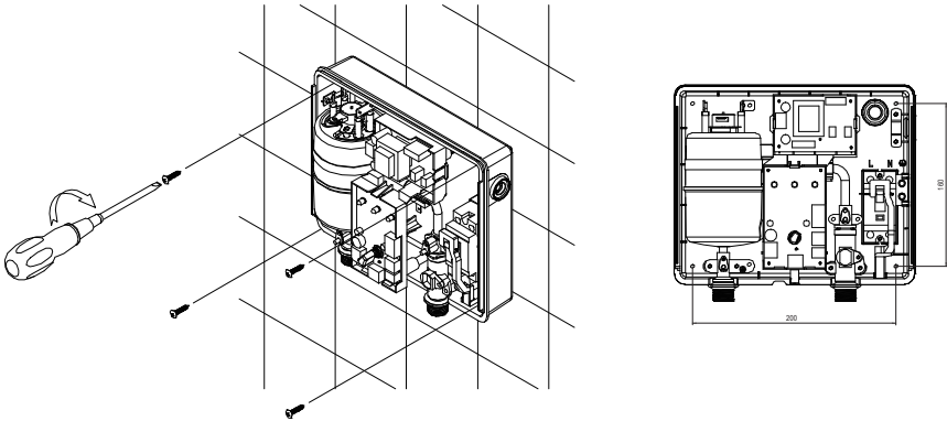
No horizontal, inverted, inclined installation! (Fig.1)
