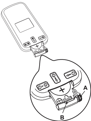
Insulation piece
